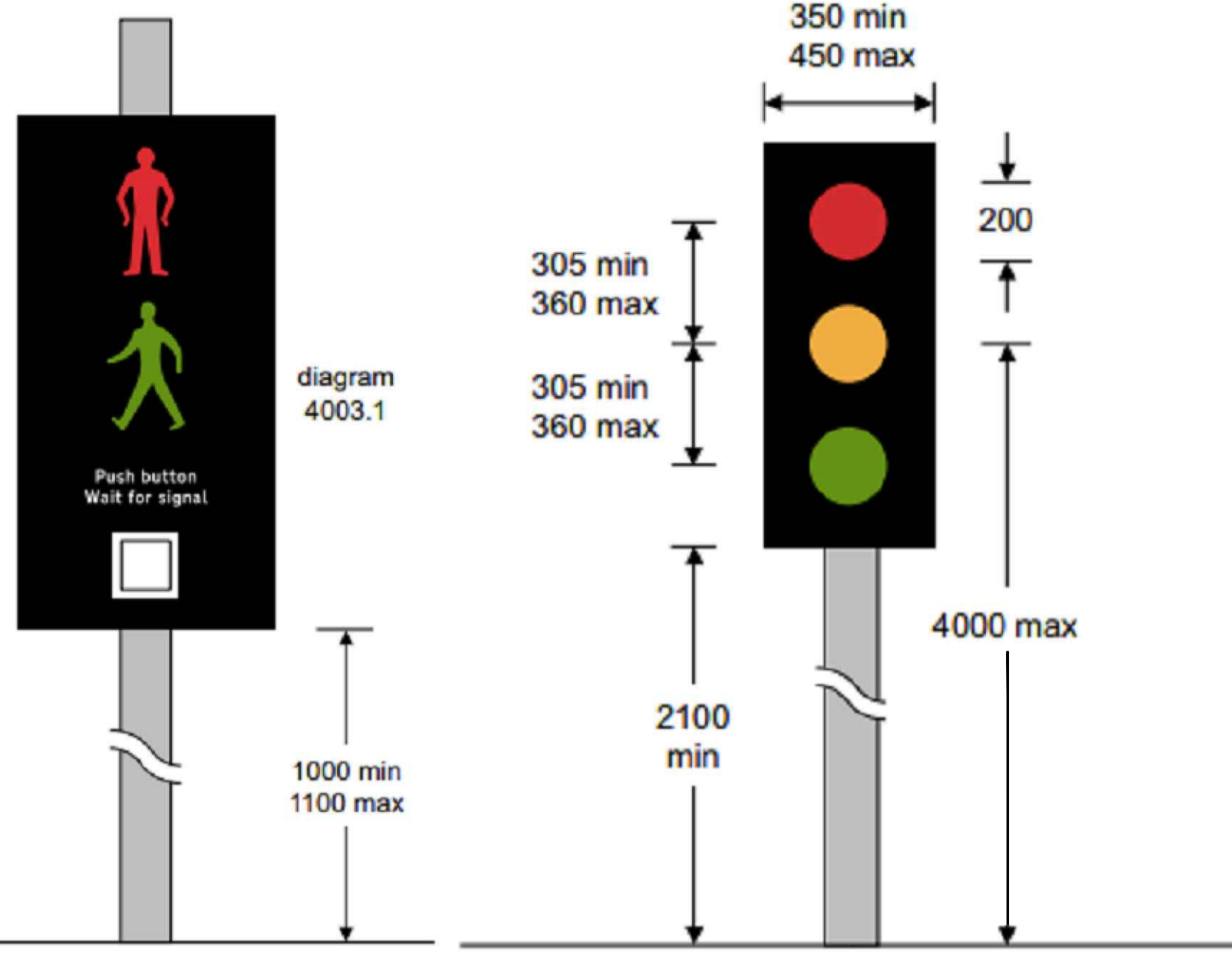
PERMANENT POLE MOUNTED PEDESTRIAN DEMAND UNIT [AKA PEDESTRIAN PUSH BUTTON] (TRAFFIC SIGNS MANUAL, CHAPTER 6, DIAGRAM 400.3.1) Not to Scale
